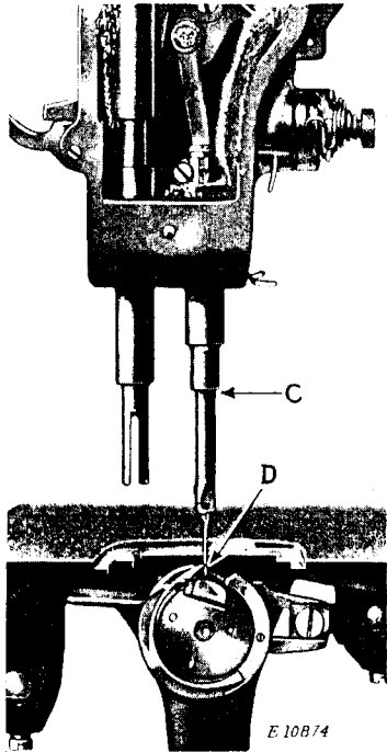
Fig. 18. Needle and Sewing Hook Correctly Timed
