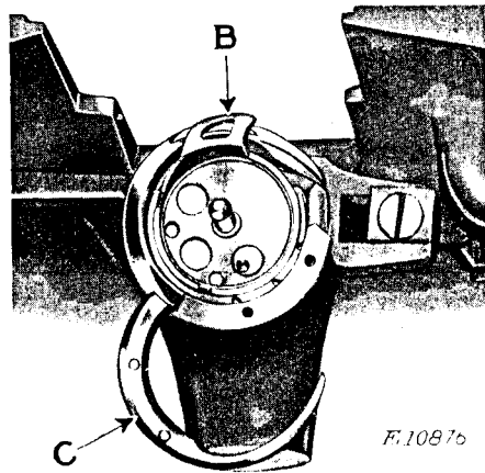
Fig. 20. Hook Gib Open for Removal of Bobbin Case Base
