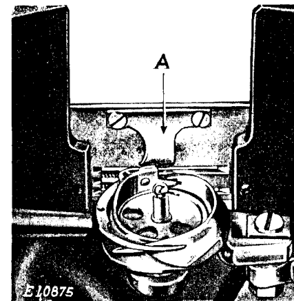
Fig. 19. Bobbin Case Base Correctly Engaged with Bobbin Case Base Stop Underneath Throat Plate
