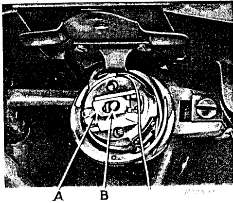
Fig. 11. Bobbin Case Threaded and Replaced
