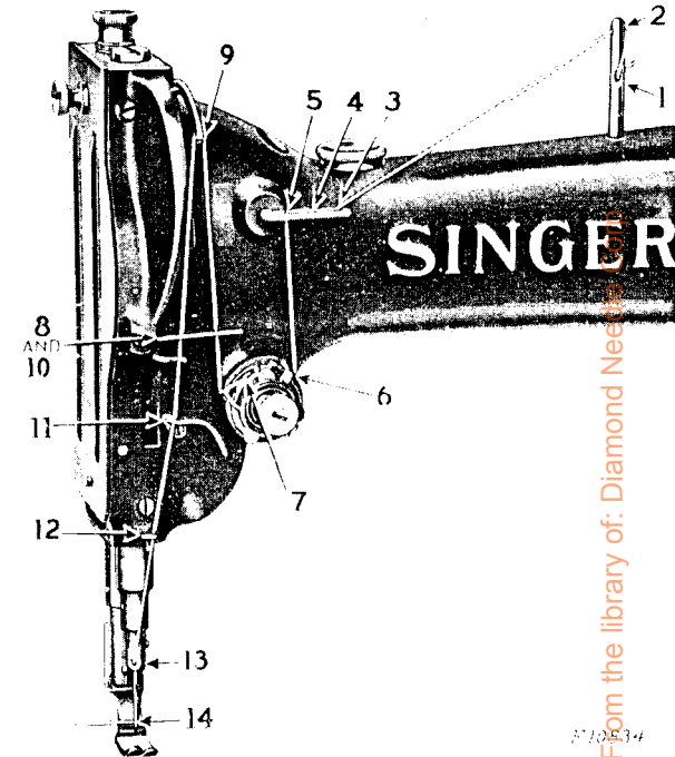
Fig. 12. Upper Threading
