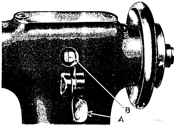
Fig. 16. Stitch Regulator
