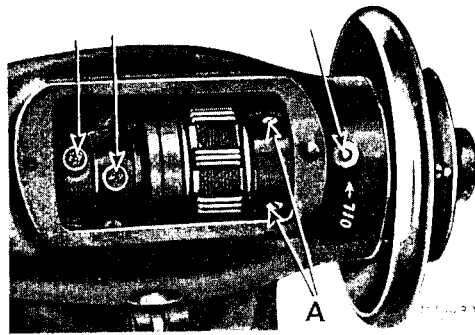
Fig. 3. Oiling Points in Arm of Machine
